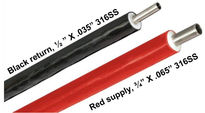
Pre-Insulated Supply/Return Tubing
