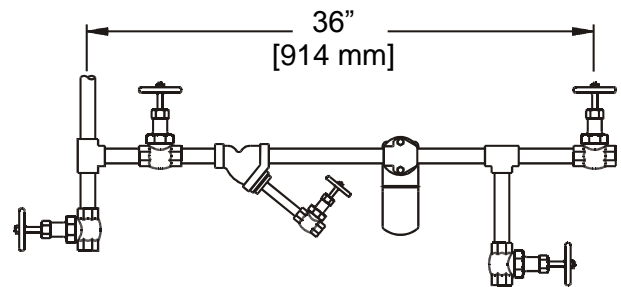
Traditional Fabricated Trap Station
