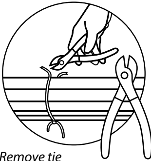
Figure 13: Remove tie wires with wire cutters
