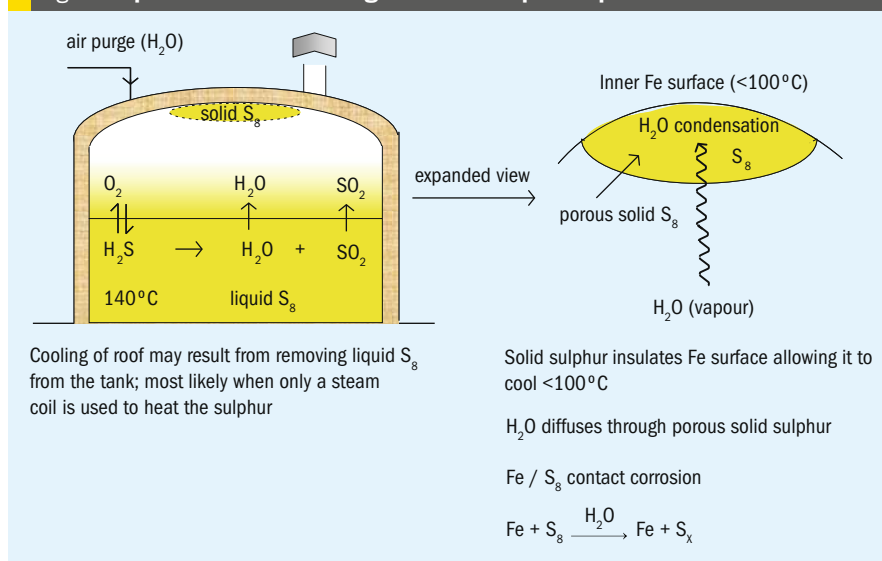
Fig 2: Sulphur corrosion resulting from solid sulphur deposition
