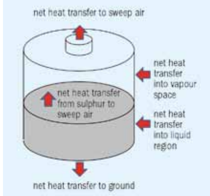
Fig 3: Model control volume and heat transfer paths
