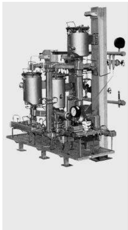
Figure 9 Bolt-On Jacketing on Polymer Additive System
