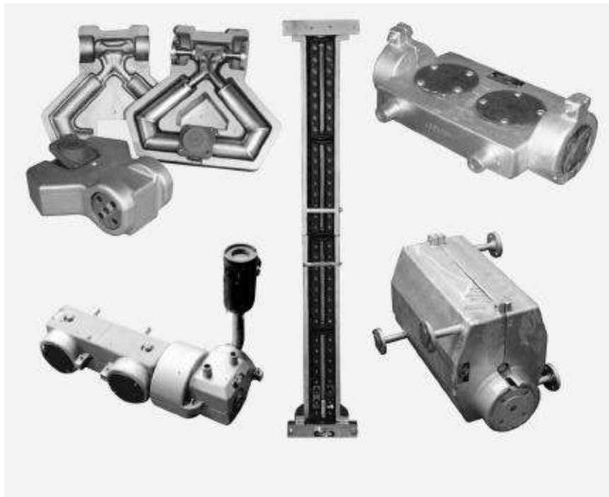
Figure 8 Bolt-On Jackets on Instrumentation
