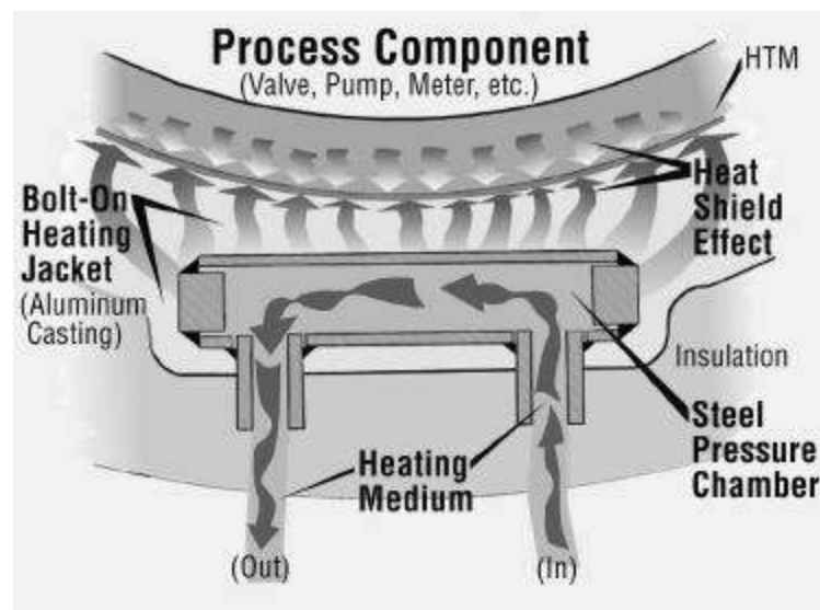
Figure 3 Heat Shield Effect
