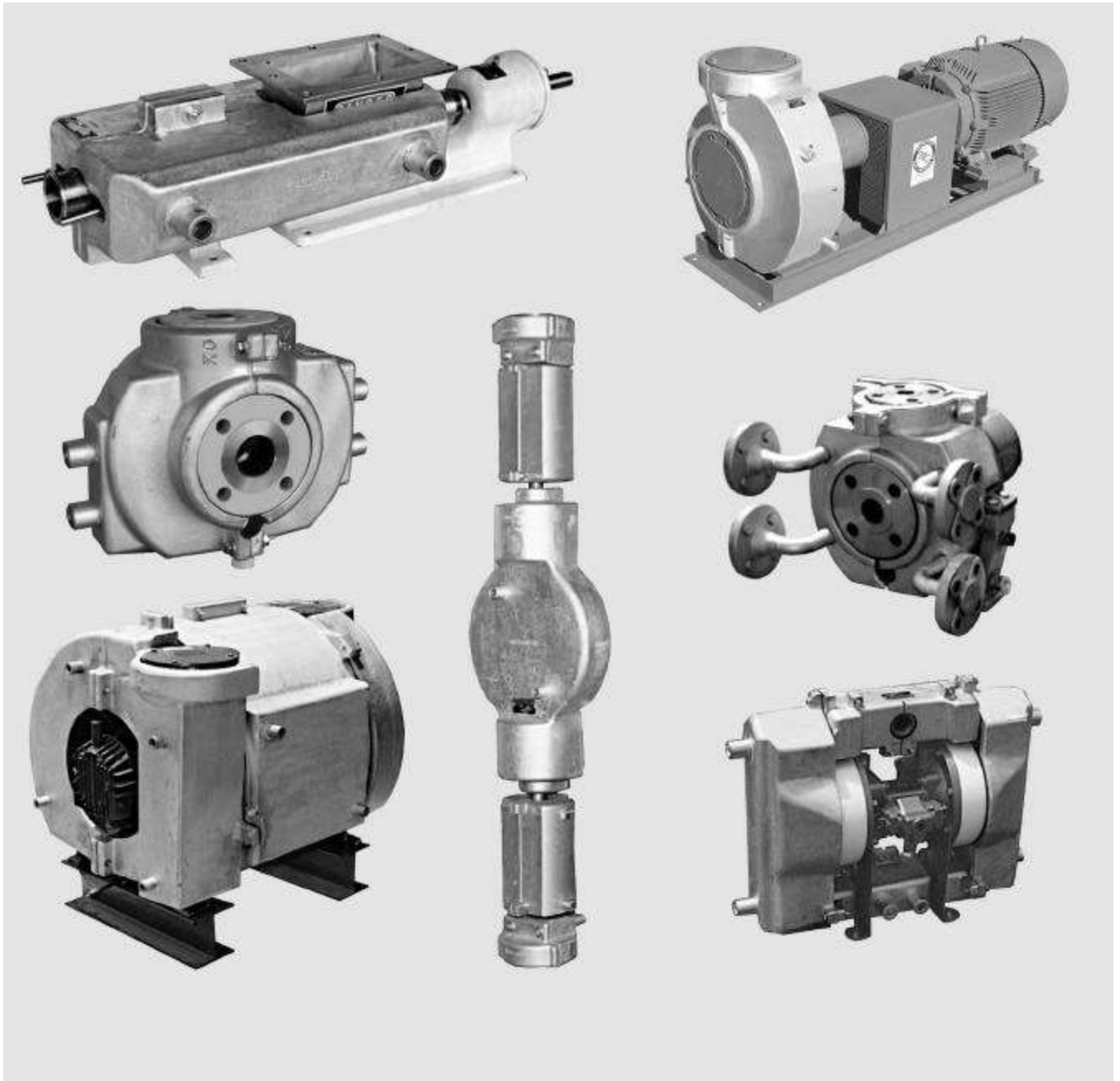
Figure 7 Bolt-On Jackets on Rotating Equipment
