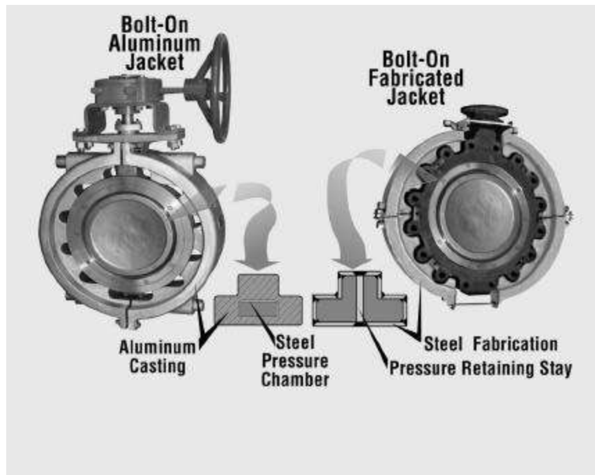
Figure 5 Cast Aluminum vs. Fabricated Bolt-On Jacket
