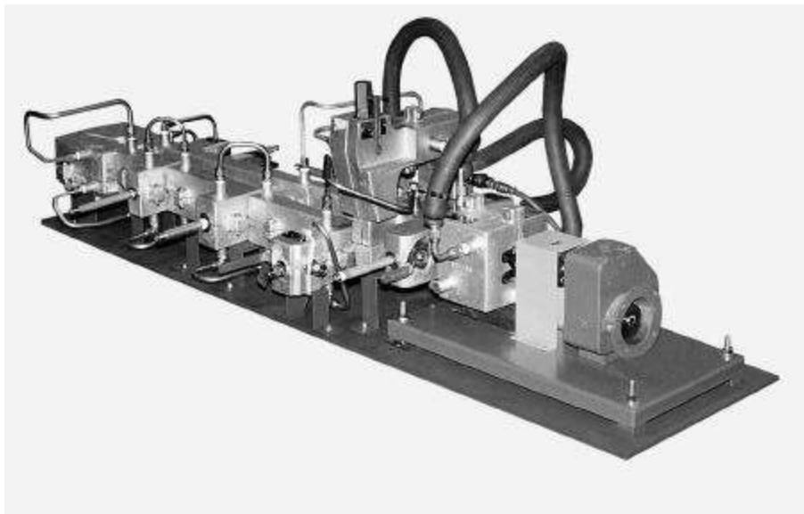
Figure 10 Bolt-On Jacketing on Valve and Metering System
